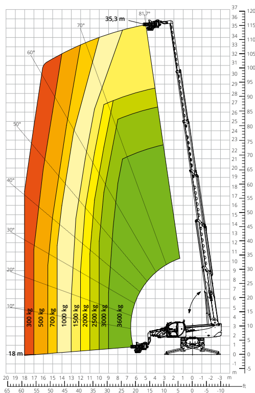
Load chart with TREE CUTTER ATT - 08 - 001
