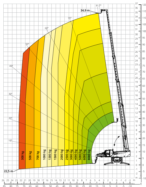
Load chart with FULLY EXTENDED STABILISERS (360°) - M2 ATT - 03 - 007
