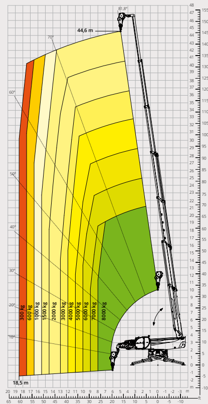
Load chart with WINCH, 8,000 kg - M2 ATT - 02 - 006
