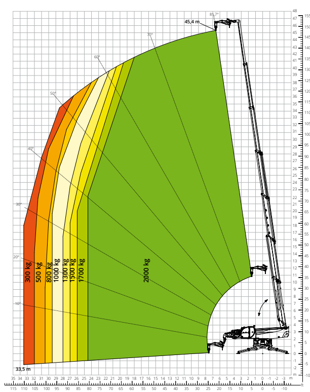
Load chart with JIB WITH WINCH, 2,000 kg ATT - 04 - 015
