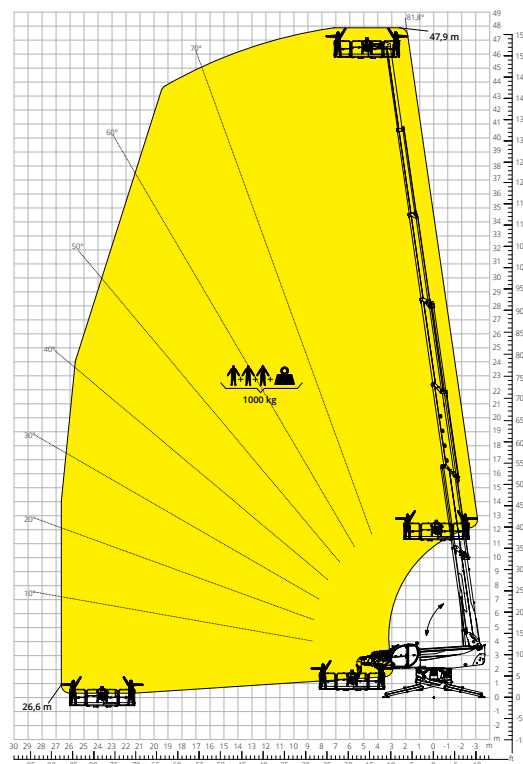
Load chart with ROTATING EXTENDABLE PLATFORM, 1,000 kg ATT - 01 - 016
