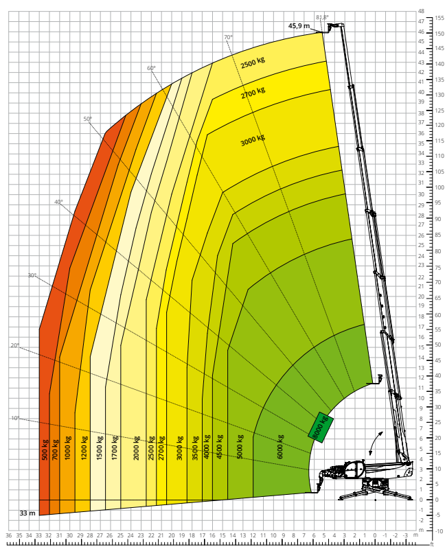
Load chart with FULLY EXTENDED STABILISERS (360°) - M1 ATT - 03 - 007
