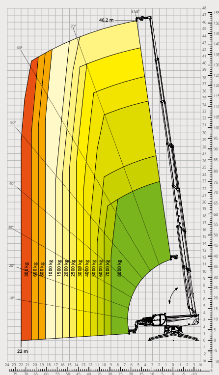
Load chart with HOOK, 8,000 kg - M2 ATT - 05 - 003
