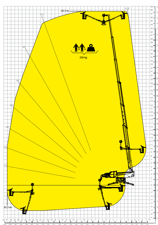
Load chart with OVER-UNDER PLATFORM - NEGATIVE ATT - 01 - 024
