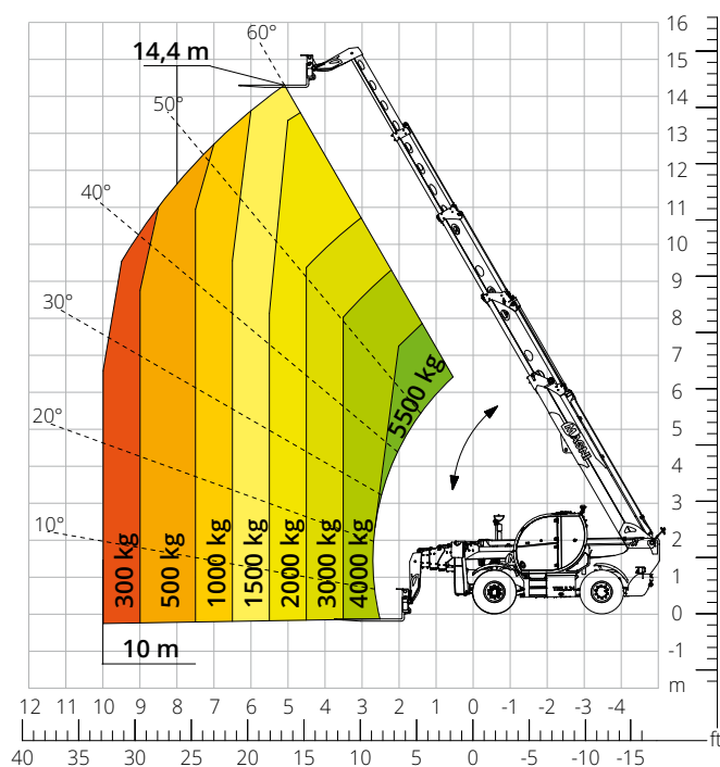
Load chart 72x72 OVERSIZED FORK CARRIAGE ON TYRES ATT-03-048
