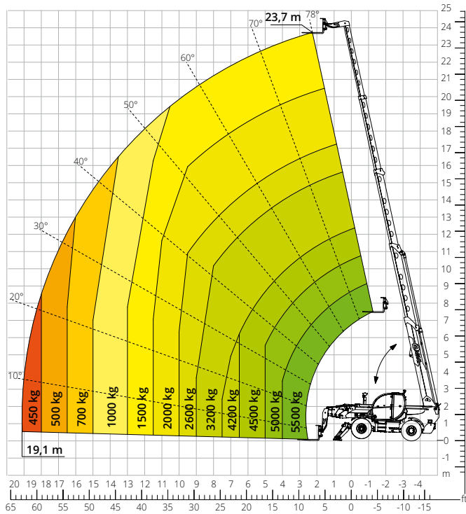
Load chart 72x72 OVERSIZED FORK CARRIAGE ON TYRES ATT-03-048
