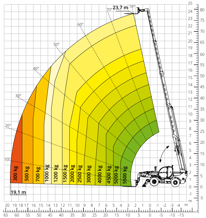
Load chart with 72x72 OVERSIZED FORK CARRIAGE ATT-03-048
