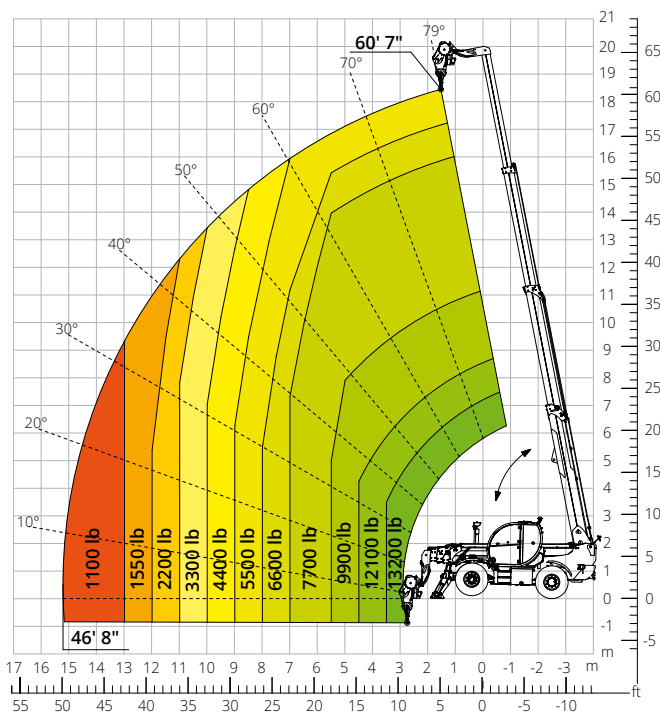
Load chart with WINCH, 13,200 lb ATT-02-004
