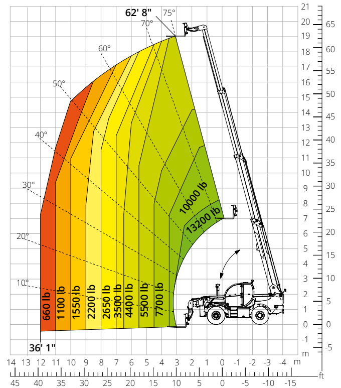
Load chart with HOOK, 13,200 lb ATT-05-001
