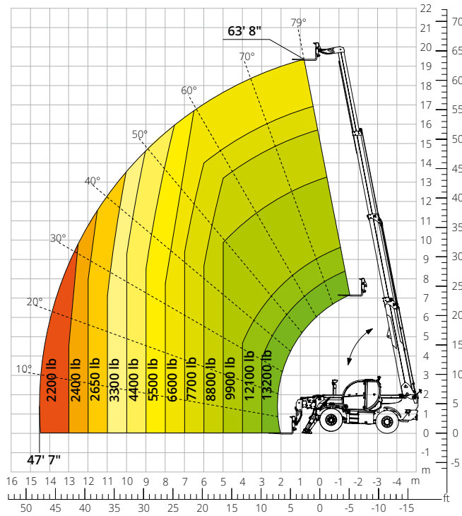
Load chart with WINCH, 13,200 lb ATT-02-004
