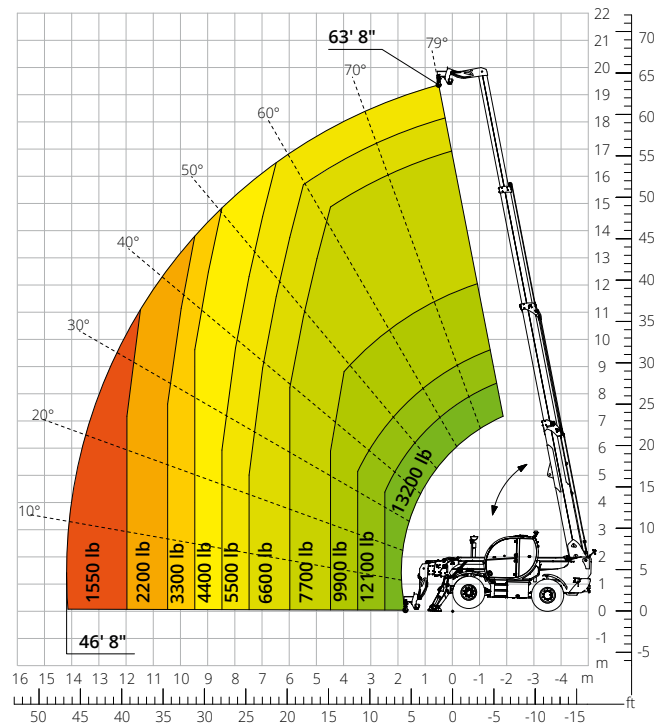
Load chart with HOOK, 13,200 lb ATT-05-001
