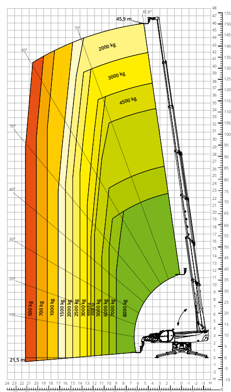
Load chart with FULLY EXTENDED STABILISERS (360°) - M2 ATT - 03 - 007
